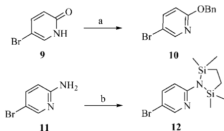
Scheme 2. Synthesis of the aglycons 10 and 12 . (a) BnBr, Ag 2 CO 3 , THF, reflux, 5 h, 93%; (b) butyllithium, Cl(Me) 2 SiCH 2 CH 2 Si(Me) 2 Cl, THF, –78 °C, 2 h, 79%.
