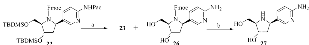
Scheme 5. Synthesis of dp2AP. (a) 1 M aq. \text{HCl}/\text{MeOH} 1:10, room temp., 30 h, 76% of 23 and 23% of 26 ; (b) piperidine, DMF, room temp., 12 h, 91%.
