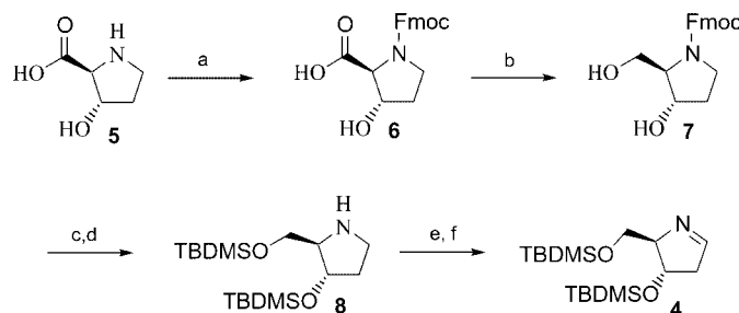
Scheme 1. Synthesis of imine 4 . (a) Fmoc-Cl, dioxane, 5% NaHCO 3 soln., 0 °C to room temp., 9 h, 98%; (b) BH 3 ·(CH 3 ) 2 S, THF, reflux, 2 h, 97%; (c) TBDMS-Cl, imidazole, THF, room temp., 2 h; (d) piperidine, THF, room temp., 12 h, 90% over 2 steps; (e) NCS, hexane, room temp., 1 h; (f) LTMP, THF, –78 °C, 2 h, 74% over two steps.
