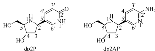
Figure 4. Numbering scheme for pyrrolidino pseudonucleosides 13–19 derived from dp2P and 20–27 derived from dp2AP used for NMR assignments.
