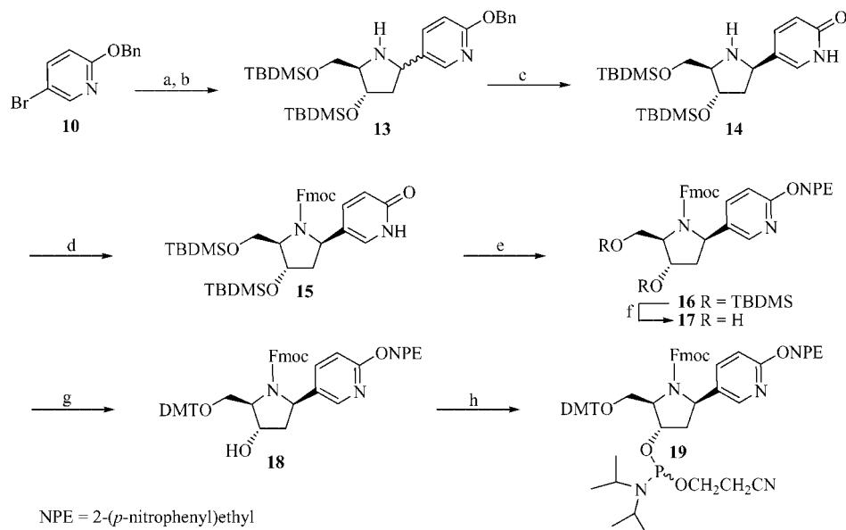
Scheme 3. Synthesis of phosphoramidite 19 . (a) Butyllithium, THF, -78^{\circ}\text{C} , 1 h; (b) 4 , THF, -78^{\circ}\text{C} ; (c) 10% Pd/C, \text{H}_2 , MeOH, room temp., 30 min., 35% over two steps; (d) Fmoc-OSu, THF, dioxane, 1 M aq. \text{NaHCO}_3 , room temp., 1 h 30, 80%; (e) \text{PPh}_3 , DIAD, p -nitrophenylethanol, dioxane, room temp., 8 h, 35%; (f) 1 M aq. \text{HCl}/\text{MeOH} 1:10, room temp., 24 h, 67%; (g) DMTCl, pyridine, room temp., 5 h, 74%; (h) \text{CEPCL} , i\text{Pr}_2\text{NEt} , THF, room temp., 2 h, 82%.
