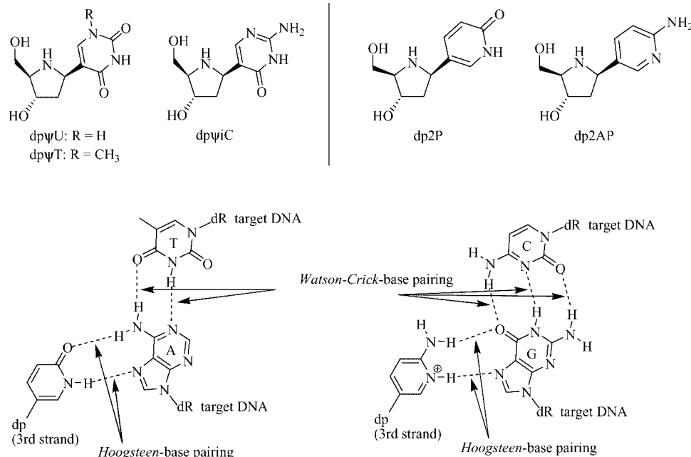
Figure 1. Top left: previously studied pyrrolidino pseudonucleoside analogues of deoxyuridine ( \text{dp}\psi\text{U} ), thymidine ( \text{dp}\psi\text{T} ) and deoxycytidine ( \text{dp}\psi\text{C} ); top right: O4 deletion mutants \text{dp}2\text{P} and \text{dp}2\text{AP} of the corresponding nucleoside analogues; bottom: expected triplex pairing patterns.
