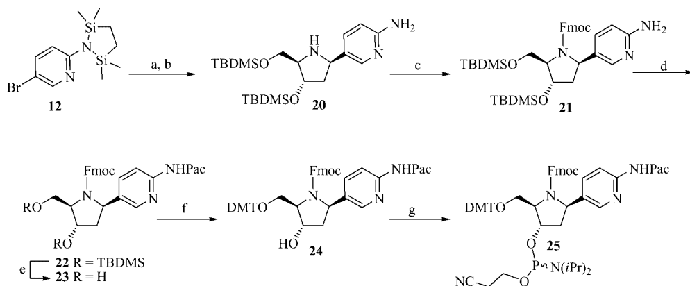
Scheme 4. Synthesis of phosphoramidite 25 . (a) Butyllithium, THF, -78^{\circ}\text{C} , 1 h; (b) 4 , THF, -78^{\circ}\text{C} , 2 h, 19%; (c) Fmoc-OSu, THF, dioxane, 1 M aq. \text{NaHCO}_3 , room temp., 30 min, 75%; (d) \text{Pac}_2\text{O} , pyridine, room temp., 2 h, 99%; (e) 1 M aq. \text{HCl}/\text{MeOH} 1:10, room temp., 24 h, 99%; (f) DMTCl, pyridine, room temp., 2 h, 88%; (g) \text{CEPCL} , i\text{Pr}_2\text{NEt} , THF, room temp., 1 h 30, 90%.
