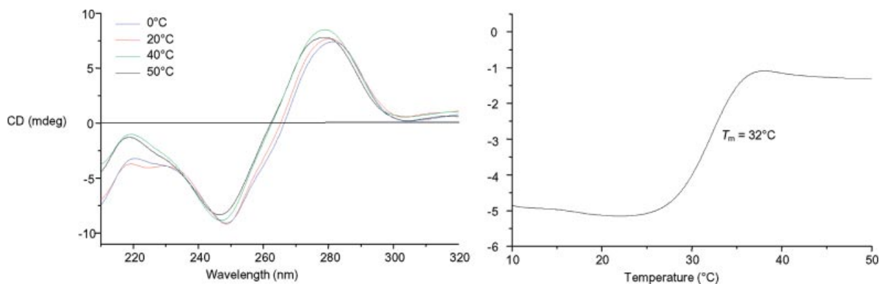
Figure 3. CD spectra of the triplex-containing TFO dp1 (Table 4); left: spectra measured at different temperatures; right: temperature scan from 10 to 50 °C at 220 nm; single strand concentration = 1.2 \mu M in 140 mM KCl, 7 mM NaH 2 PO 4 , 0.5 mM MgCl 2 , pH 6.0.
